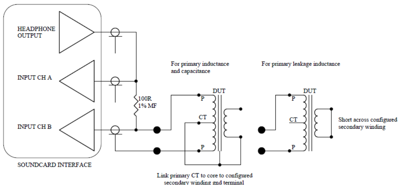
Figure 2. Soundcard connections for Impedance measurement
