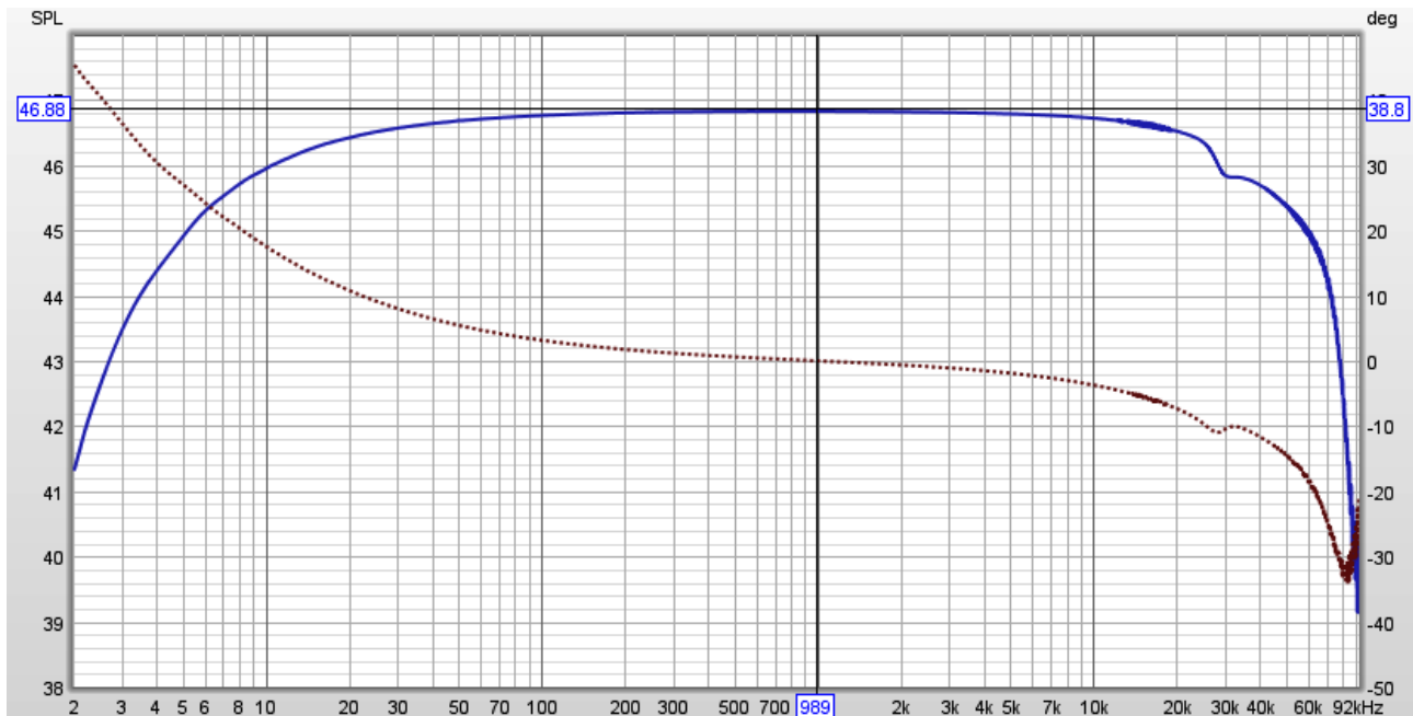
Figure 21. Frequency response of OP25 (old) with 3.75\Omega secondary configuration and load
