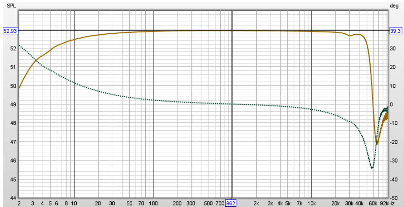
Figure 24. Frequency response of OP25 (new) with 15 \Omega secondary configuration and load
