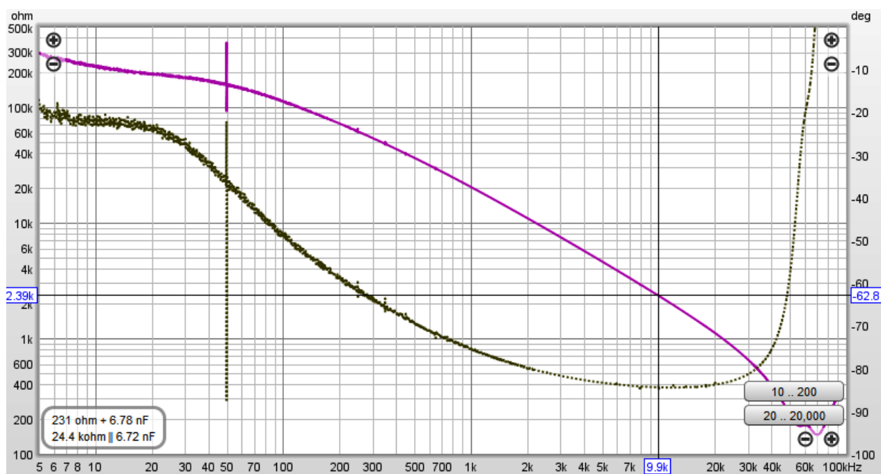
Figure 17. Shorted primary to shorted secondary impedance for Red Line AF8/2
