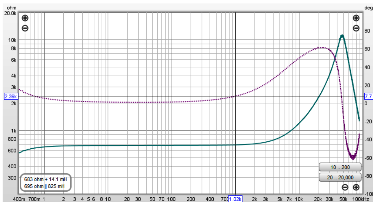
Figure 11. Shorted secondary impedance for WWFB in 3.8Ω configuration
