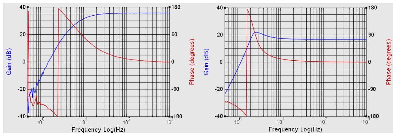
Figure 30. AF8/2 - 8Ω low frequency gain and phase responses without and with feedback.
