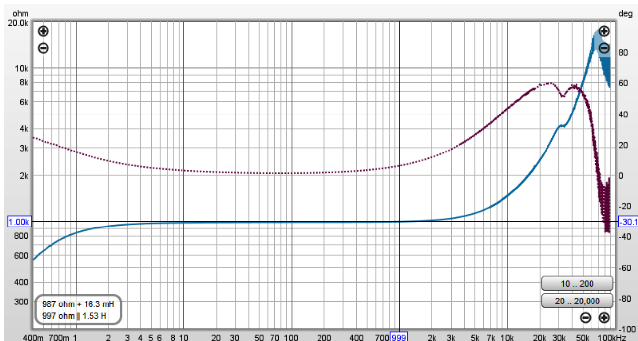
Figure 12. Shorted secondary impedance for Ferguson OP25 (new) in 4Ω configuration
