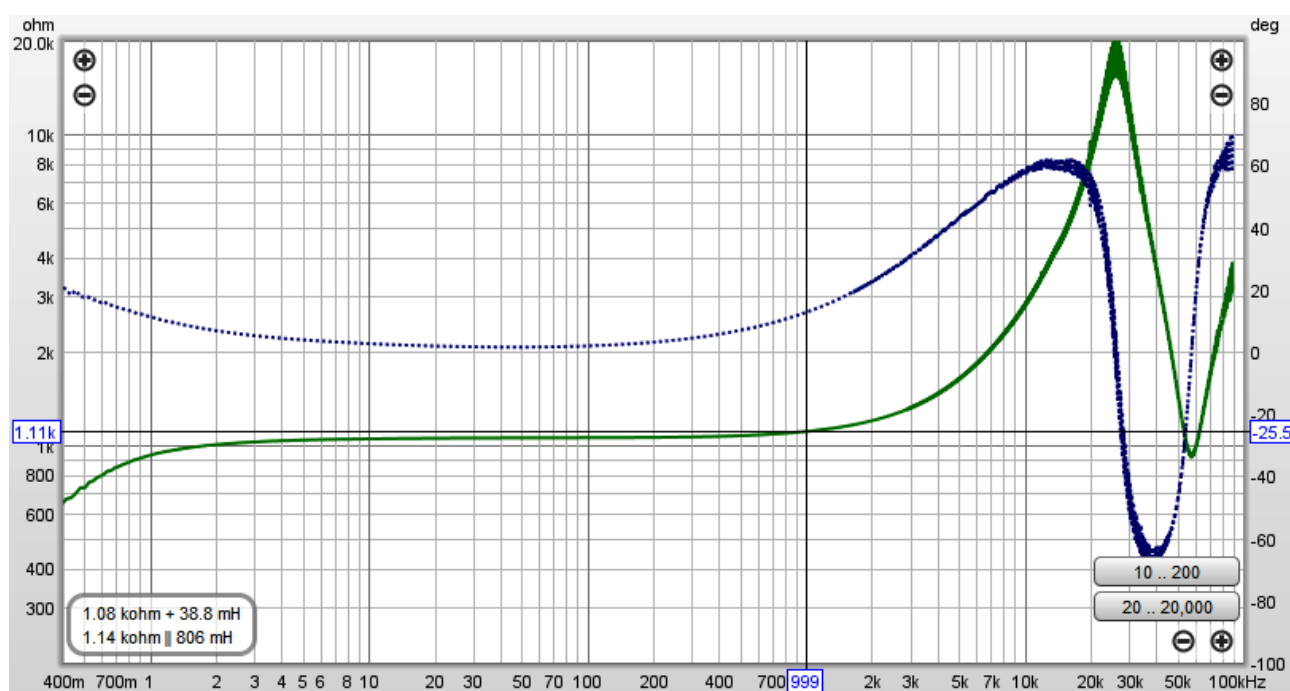
Figure 13. Shorted secondary impedance for Red Line AF8/2 in 8R configuration
